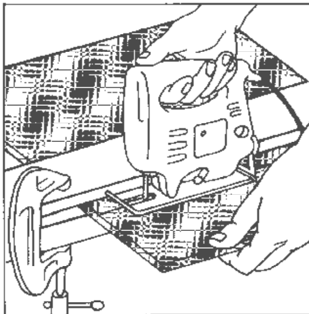
Use clamping strip as a guide for the saw.
